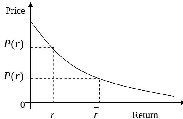
Figure 7.1. The dependence of the bond price on the return r .
