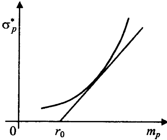
Figure 8.3. The dependence of the optimal portfolio risk on its return.
