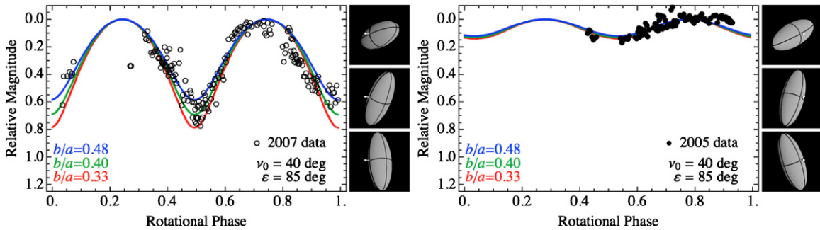
Figure 9. Same as Figure 6 but for obliquity \varepsilon = 85^\circ , solstice position \nu_0 = 40^\circ , and ellipsoids with axis ratios b/a = 0.33 (red), b/a = 0.40 (green), and b/a = 0.48 (blue).
