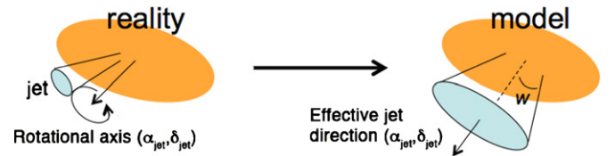
Figure 10. Schematic diagram showing how a near-polar jet of directed ejected material can be approximated by a wider jet with an effective orientation equivalent to the direction of the rotational pole itself.
