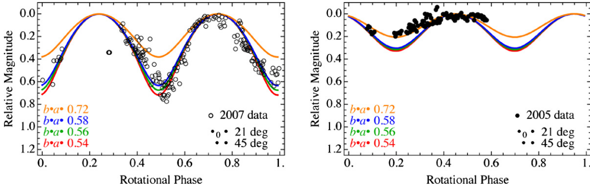
Figure 8. Same as Figure 6 but for obliquity \varepsilon = 45^\circ and an ellipsoid with axis ratio b/a = 0.72 (solid orange line). (A color version of this figure is available in the online journal.)
