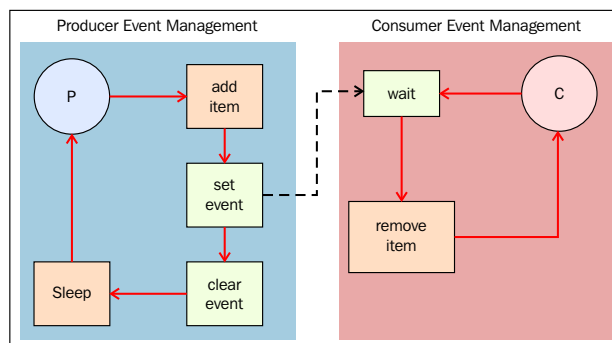
Thread synchronization with event objects
