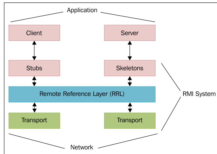
Remote Method Invocation
