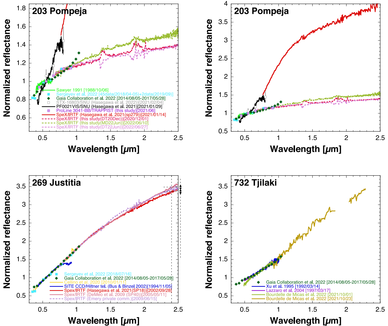
Figure 5. Spectra of 203 Pompeja (top panels), 269 Justitia (bottom left panel), and 732 Tjilaki (bottom right panel). Square brackets in these panels indicate the observation dates. Black arrows are present on the right-hand side of the vertical axis in the 269 figure. Arrows indicate the slope uncertainty from Marsset et al. (2020) centered at the reflectance value of the spectra at 2.40 \mu\text{m} , as shown by the black dashed lines.
