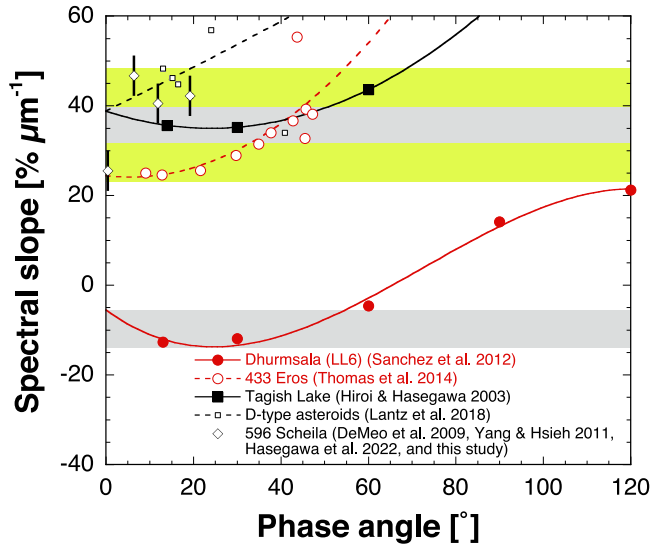
Figure 3. Comparison between the spectral slopes of the Dhurmsala (LL6) and Tagish Lake (C2) meteorites, Sw-type asteroid 433 Eros, and D-type asteroids as a function of phase angle. The D-type asteroid data set is a combination of multiple D-type asteroids. Gray and yellow areas indicate the slope uncertainty from Marsset et al. (2020) for the meteorites and asteroids, respectively. The solid and dashed lines represent polynomial fits for the meteorites and asteroids, respectively. The D-type data set includes the postimpact spectrum of 596.
