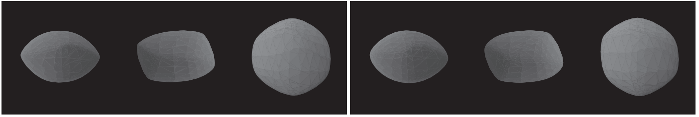
Figure A1. Convex shape models of 203 Pompeja. While the left panel represents the pole solution \lambda_1 = 315 [deg], \beta_1 = -40 [deg], the right panel shows the pole solution \lambda_2 = 132 [deg], \beta_2 = -36 [deg]. The left and middle views are equatorial with a 90^\circ rotation, while the right view is pole-on. Both shape models appear very similar.
