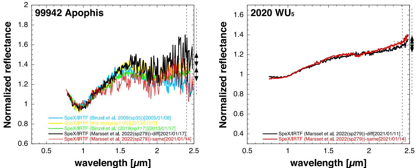
Figure B1. Spectra of 99942 Apophis (left panel) and 2020 WU 5 (right panel). The data of 203 Pompeja, 99942 Apophis, and 2020 WU 5 were taken on 2021 January 14. The spectra of 99942 and 2020 WU 5 were measured four times and once, respectively (Binzel et al. 2009, 2019; Marsset et al. 2022), in addition to their measurement on the same day as 203 (Hasegawa et al. 2021). The five spectra of 99942 and the two spectra of 2020 WU 5 are found to be in agreement. Square brackets in these panels indicate the observation dates. The black arrows indicate the slope uncertainty from Marsset et al. (2020) centered at the reflectance value of the spectra at 2.40 \mu\text{m} , as shown by the black dashed lines.
