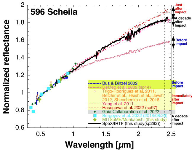
Figure 2. Comparison of 596 Scheila’s NIR spectra before, immediately after, and a decade after the 2010 impact event. The figure shows spectra of 596 in the 0.4–2.5 \mu\text{m} wavelength region, normalized to 1 at 0.55 \mu\text{m} . The black arrows indicate the slope uncertainty from Marsset et al. (2020) centered at the reflectance value of the spectra at 2.40 \mu\text{m} , as shown by the black dashed lines.
