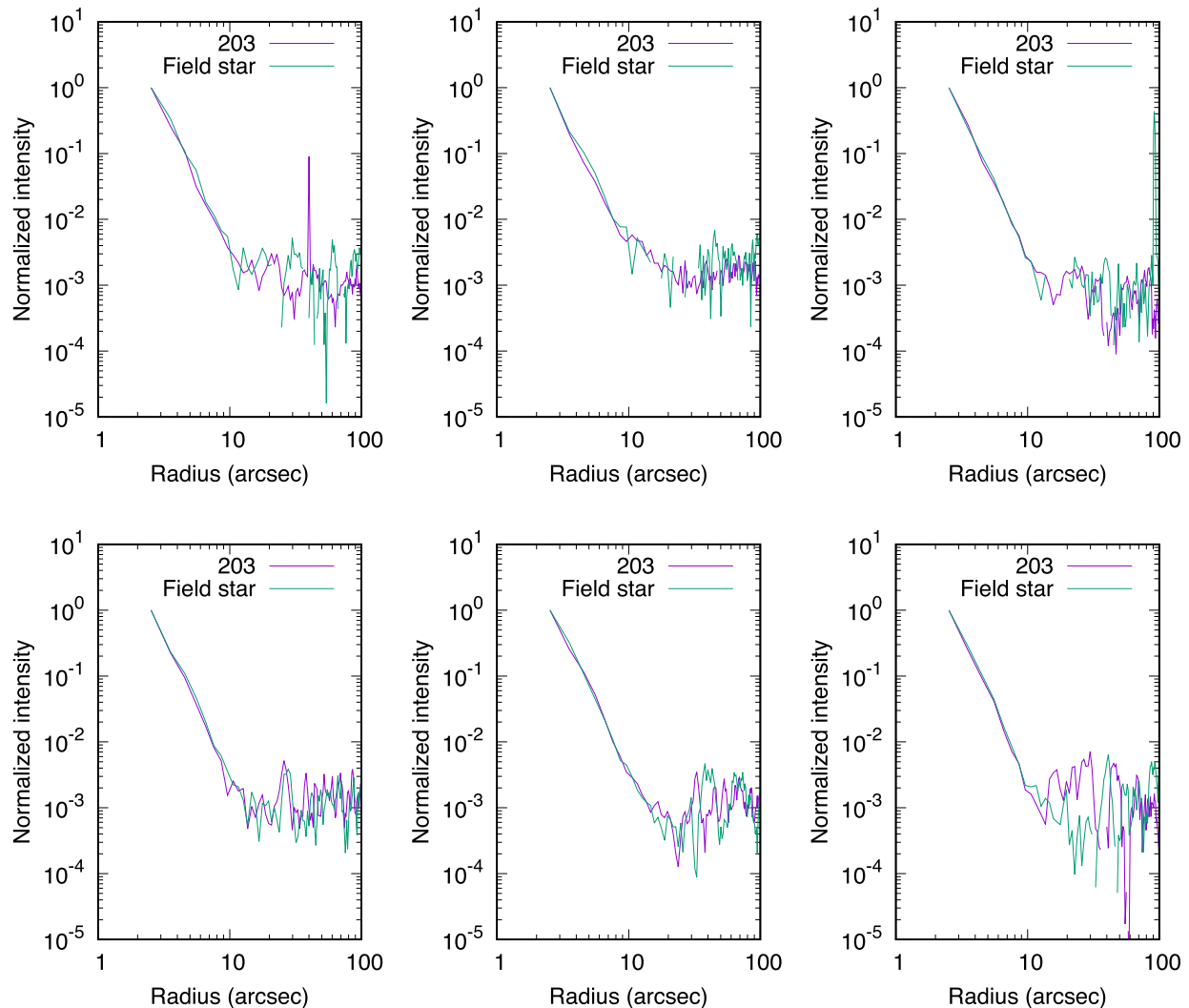
Figure D1. Radial brightness profiles of 203 Pompeja obtained by the Zwicky Transient Facility on 2020 December 10 (top left), 17 (top middle), and 22 (top right) and 2021 January 5 (bottom left), 13 (bottom middle), and 19 (bottom right). These profiles are normalized at 2''.5 from the photocenter and compared with field stars. The FWHM of the images used was roughly 2'' – 3'' . Since 203 was almost saturated, brightness profiles within 2''.5 from the photocenter are not given.
