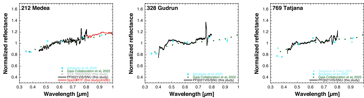
Figure C1. Spectra of 212 Medea, 328 Gudrun, and 769 Tatjana. The spectra of these asteroids were obtained at SAO in 2020–2021. Previous spectra were derived from Sergeyev & Carry (2021), Sergeyev et al. (2022), and Gaia Collaboration et al. (2022).
