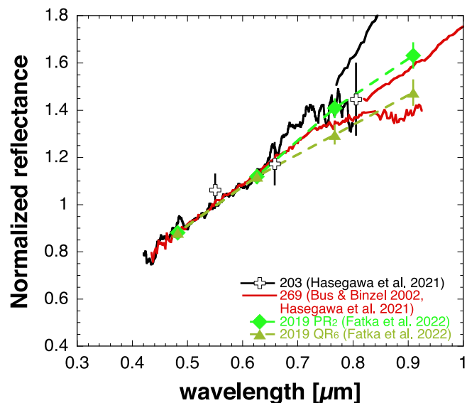
Figure 1. Comparison of the visible spectra of VROs 203 Pompeja, 269 Justitia, 2019 PR 2 , and 2019 QR 6 . The figure shows the spectra in the 0.4–1.0 \mu\text{m} wavelength regions, normalized to 1 at 0.55 \mu\text{m} .
