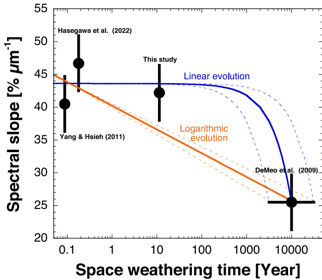
Figure 4. Spectral slope for 596 Scheila against space weathering time. Blue and orange lines correspond to linear and logarithmic regression of the spectral slope values of DeMeo et al. (2009), Yang & Hsieh (2011), and Hasegawa et al. (2022), respectively.
